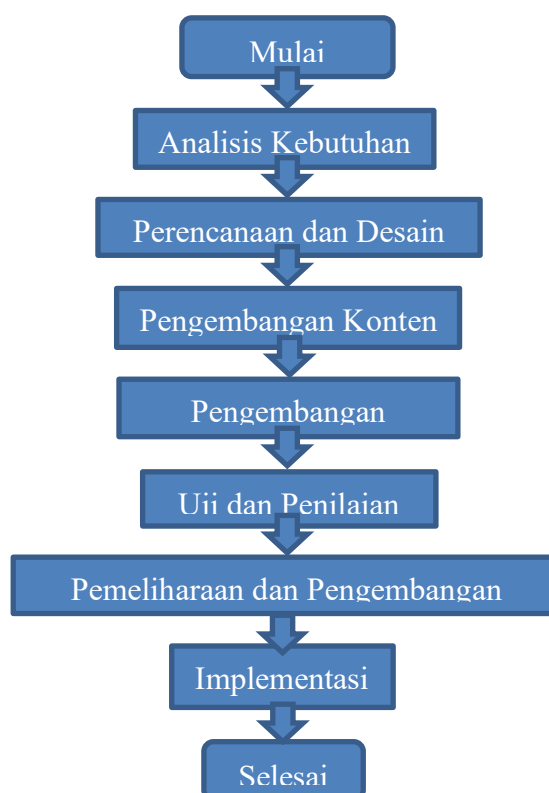
Gambar 2. Alur Penelitian
