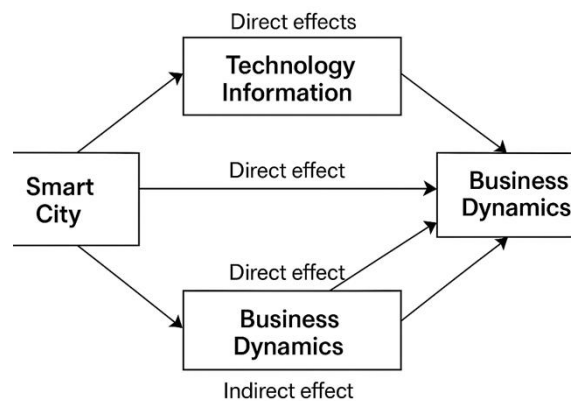
Figure 1. Research Model.
